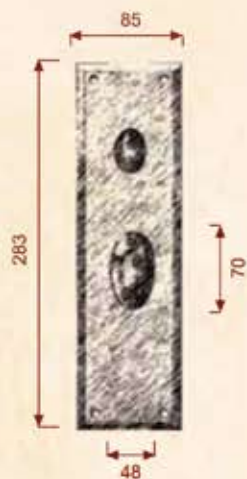
ALP4010-ML09-50 (Mortise Lock)
