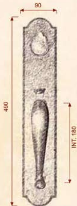
ALP3010-ML09-50 (Mortise Lock)
