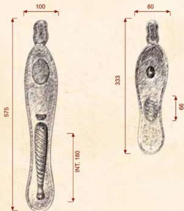
ALP5010-MT09-55 (Mortise Lock)
