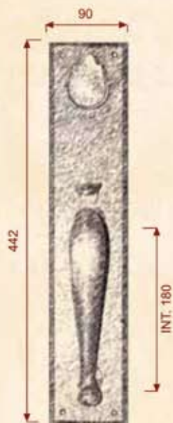
ALP4010-ML09-50 (Mortise Lock)
